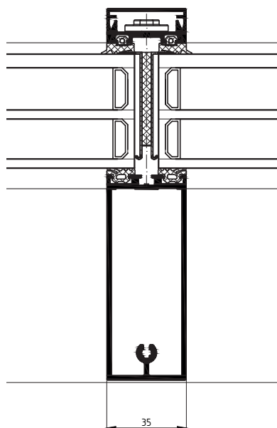
Schüco facade FWS 35 PD
