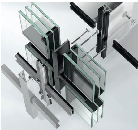
Schüco facade FWS 35 PD
